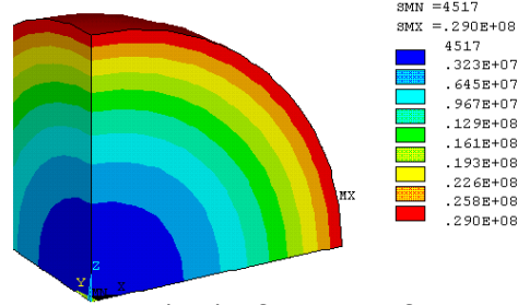
Temperature distribution ( ^\circ\text{C} ) and von Mises stress (Pa) after 1 s of cooling
