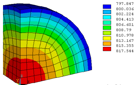
Temperature distribution ( ^\circ\text{C} ) and von Mises stress (Pa) after 1 s of cooling
