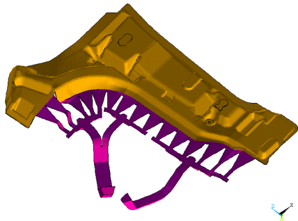
FE model
