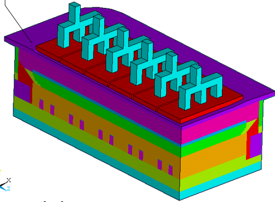
Corner model
