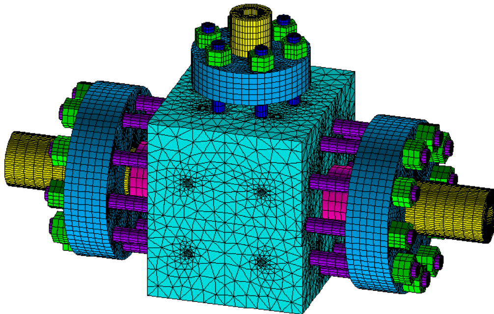
FE model
