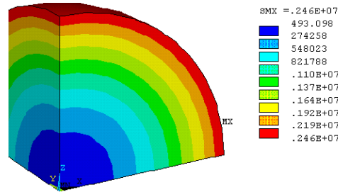
Temperature distribution ( ^\circ\text{C} ) and von Mises stress (Pa) after 46 seconds of cooling
