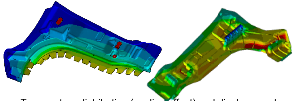
Temperature distribution (cooling effect) and displacements
