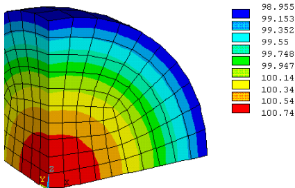
Temperature distribution ( ^\circ\text{C} ) and von Mises stress (Pa) after 46 seconds of cooling
