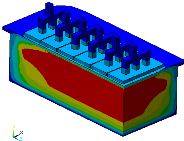
Temperature distribution
